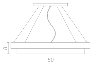
Ref. 1210 L - 50 cm A - 8 cm P - 50 cm Placa de LED
