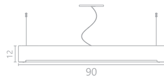
Ref. 477 L - 90 cm A - 12 cm P - 20 cm
