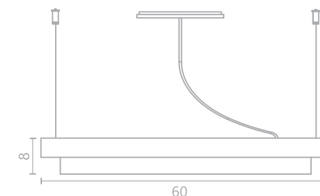
Ref. 1211 L - 60 cm A - 8 cm P - 30 cm Placa de LED
